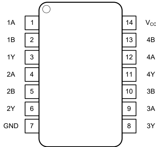
Fig. 4. Top view pin configuration SOP and TSSOP
