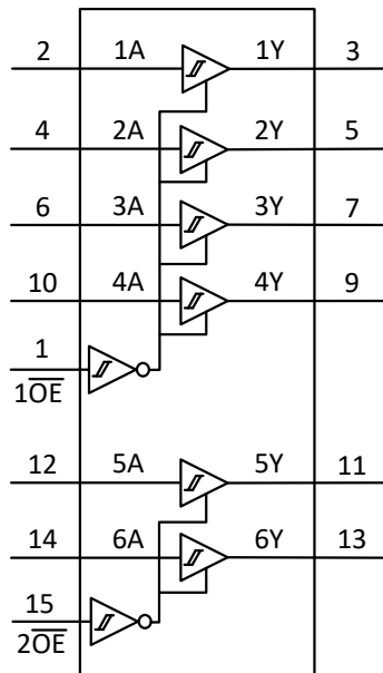
Fig. 1. Functional diagram
