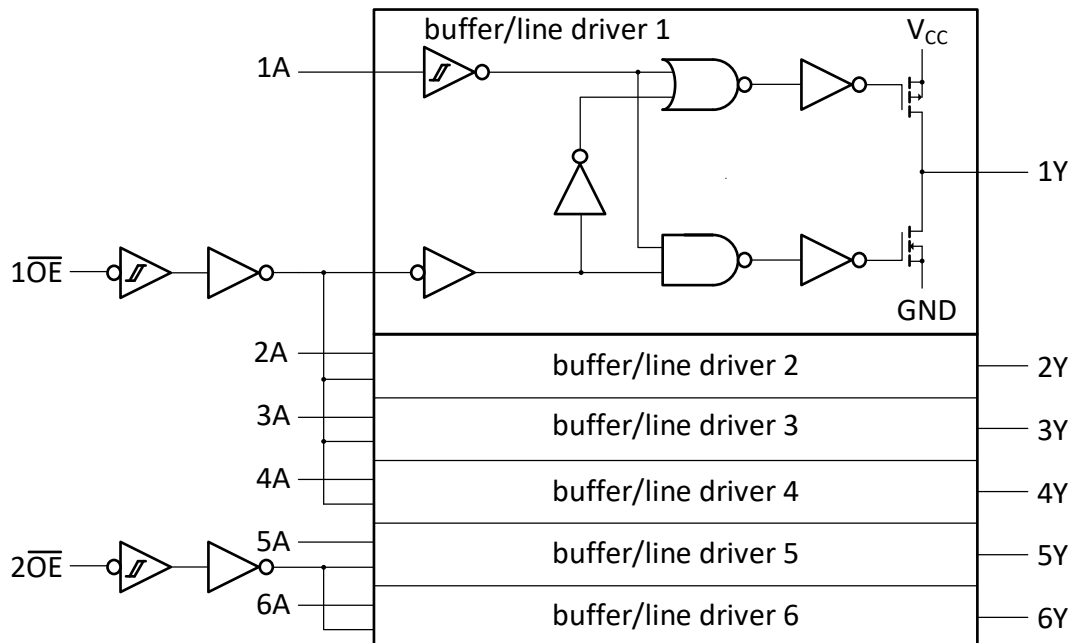
Fig. 3. Logic diagram
