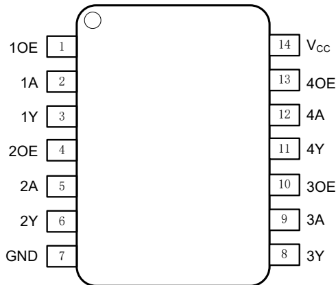
Fig. 4. Top view pin configuration SOP and TSSOP
