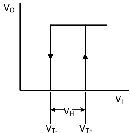
Fig. 14. Transfer characteristic
