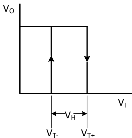
Fig. 12. Transfer characteristic
