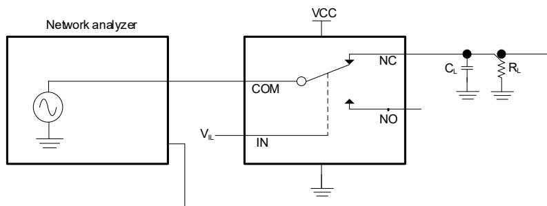
Fig 5. Bandwidth
