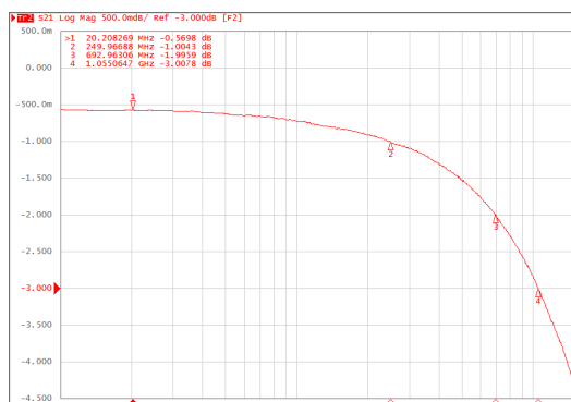
Fig 3. Bandwidth
