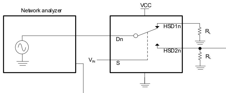
Fig 7. Off isolation
