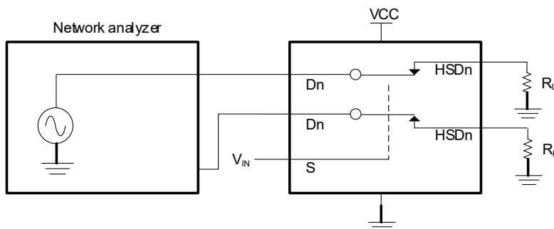
Fig 8. Crosstalk
