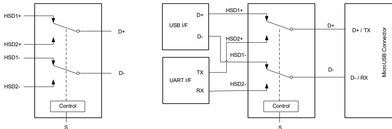
Fig 3. USB2.0 Switch
