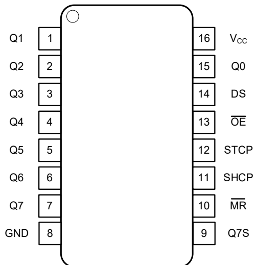
Fig. 5. Top view pin configuration SOP and TSSOP
