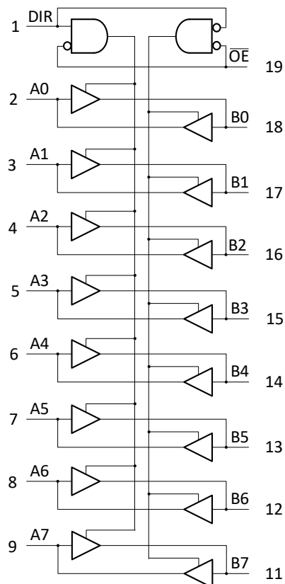
Fig. 1. Logic symbol
