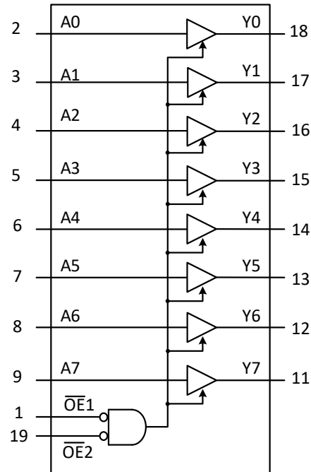
Fig. 3. Functional diagram
