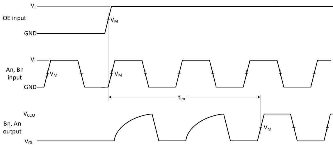
Fig. 3. The data input (An, Bn) to data output (Bn, An) propagation delay times
