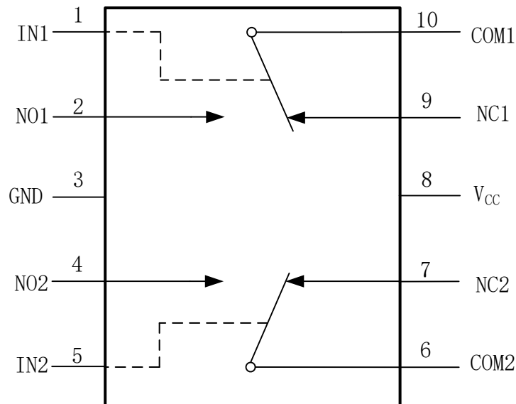
Fig 2. Analog Symbol
