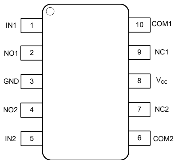
Fig 1. Top view pin configuration MSOP-10L
